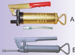
MGM -1201 GREASE GUN A) 285cc/ 8 Oz./ 5/16" PISTON B) 4 Oz., 1/4" PISTON
