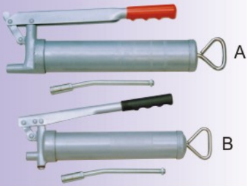
MGM -1200 GREASE GUN A) 445cc/ 15 Oz./ 1/2" PISTON B) 445cc/ 15 Oz./ 5/16" PISTON
